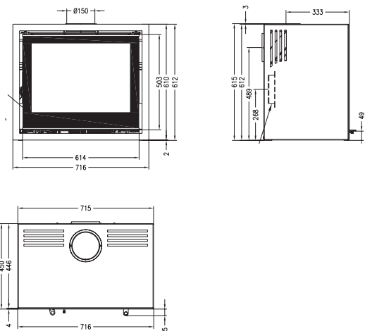
LINEAR Module M incl. Base B WxHxD 716x978x450 mm
